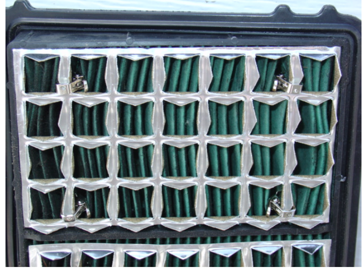
Small clamps are used to securely attach Eco Charge ICB to the filter.
