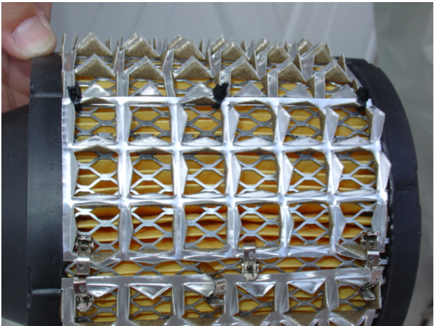
The sheets are attached with clamps after cut to size
